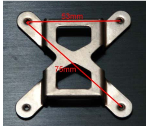
HR-03 Mounting Bracket
